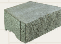
Gradino™ Wall 406x305x152mm • 15.98x12.01x5.98"
