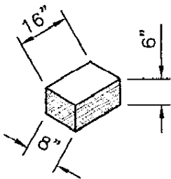
CORNER BLOCK
