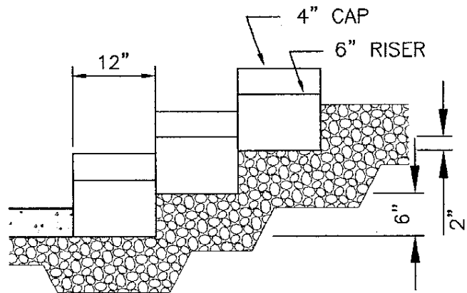
STAIR ELEVATION
