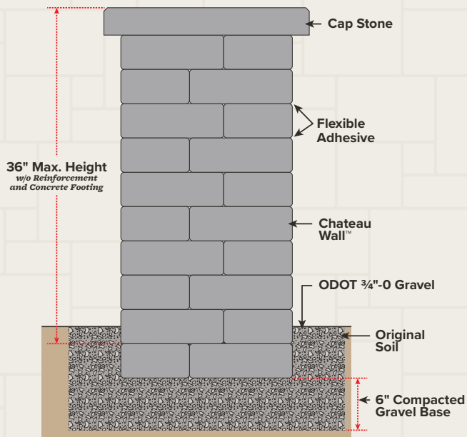
Free-standing 20" Column
